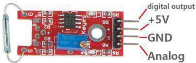
Reed Switch
