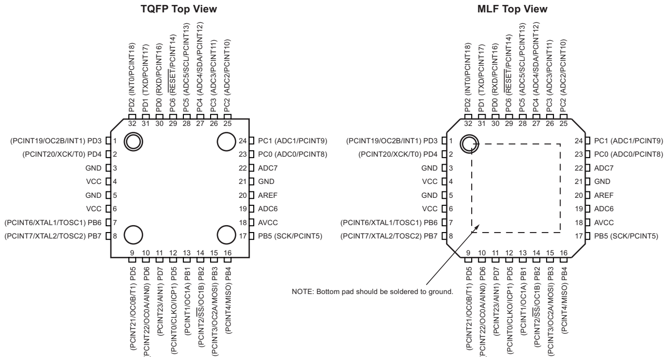
Figure 1-1. Pinout ATmega88/168
