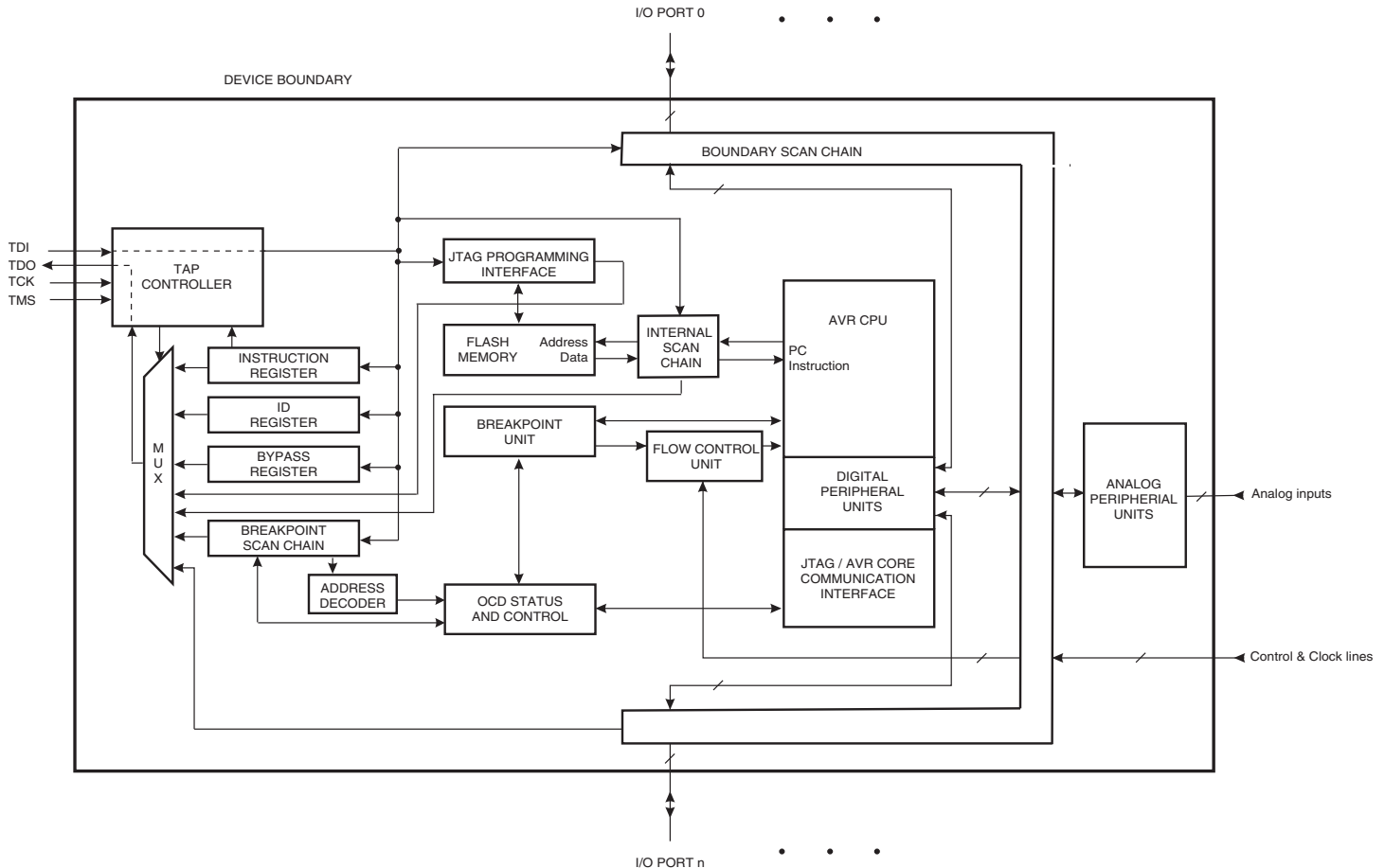
Figure 27-1. Block Diagram
