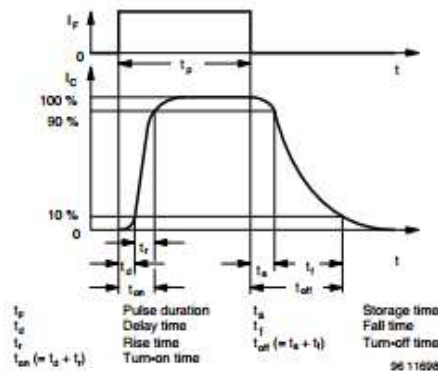
Fig. 5 - Switching Times
